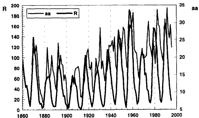
Fig. 5 Yearly values of the sunspot number R and the geomagnetic activity index aa
