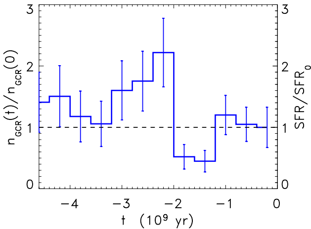
Fig. 2 Histogram of the star formation rate (SFR), adapted from Rocha-Pinto et al. (2000a, 2000b), and the variation in Cosmic Rays (CR) in the Milky Way (see text). Both are normalized to present day values. The temporal resolution is 0.4 Gyr.
