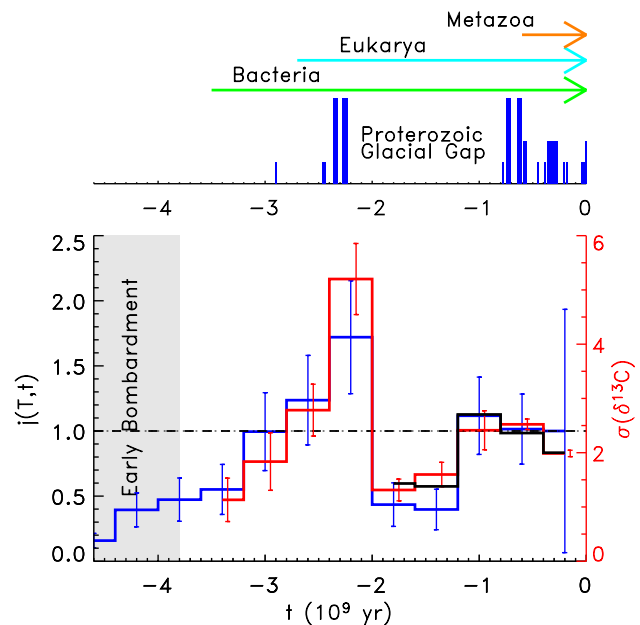
Fig. 5 Upper panel show periods of glaciations (blue bars), and arrows are the temporal extend of major life forms. Bottom panel: CR levels or Standard deviation of CR fluctuations \sigma_{\text{CR}} with energy 10 GeV at 1 AU over 4.6 billion yr (blue curve) and over 2 billion years (black curve). Standard deviation of \delta^{13}\text{C} fluctuations \sigma(\delta^{13}\text{C}) (red curve), all curves in time steps of 0.4 Gyr years (correlation coeff. = 0.92). SFR data based on data from de la Fuente Marcos & de la Fuente Marcos (2004) (black curve). The grey area represent the time when the Earth's was heavily bombarded by asteroids and comets.
