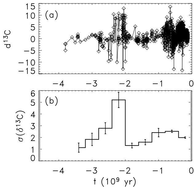
Fig. 4 (a) \delta^{13}\text{C} record from carbonate sediments over almost 4 billion years. (b) Fluctuations \sigma(\delta^{13}\text{C}) averaged over 0.4 Gyr time steps.
