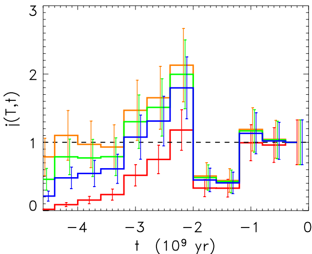
Fig. 3 Variation of CR at 1 AU with energies of 1 GeV (red), 5 GeV (blue), 10 GeV (green) and 20 GeV (orange). Note that the higher solar activity of the young sun reduced the heliosphere of cosmic rays. The temporal resolution is 0.4 Gyr.
