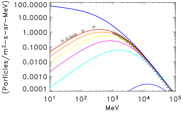
Fig. 1 Differential energy spectrum of cosmic rays at Earth as a function of solar evolution. Red curve ( t = 0 Gyr), brown ( t = -0.5 Gyr), yellow ( t = -1.3 Gyr), purple ( t = -2.1 Gyr), turquoise ( t = -2.9 Gyr), and blue ( t = -3.8 Gyr). Note that the low energies of CR gets depleted. The diamonds and triangles are present day observations, see text.
